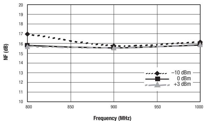
Figure 6. Noise Figure vs Frequency and LO Power @ 900 MHz
