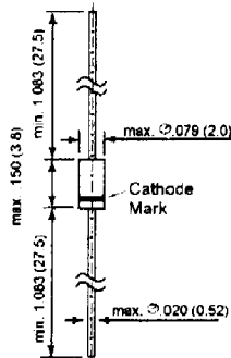
DO-35
