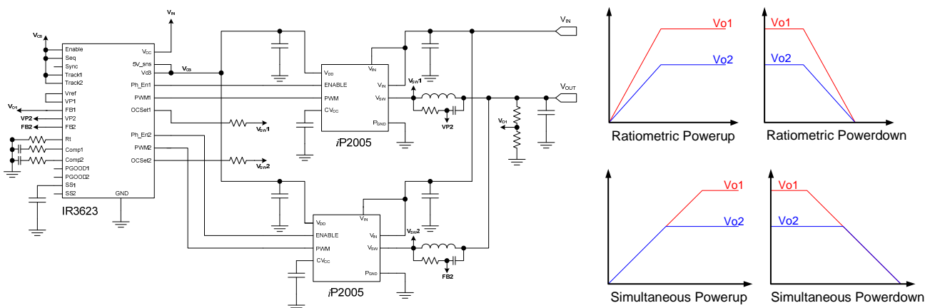
Fig. 1: Power Up /Down Sequencing
