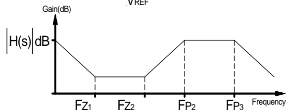
Fig. 20: Compensation network with local feedback and its asymptotic gain plot
