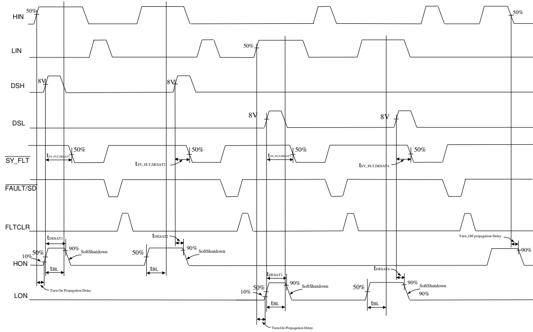
Figure 10: Desat Timing
