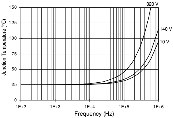
Figure 30. IRS2112 T J vs. Frequency (IRFBC40) R GATE = 15 Ω, V CC = 15 V
