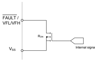
Figure 3: FAULT/N, VFH, VFL diagram
