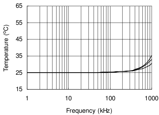
Figure 22. IRS2011S vs. Frequency (IRFBC20) R_{gate}=33 \Omega , V_{CC}=12 V
