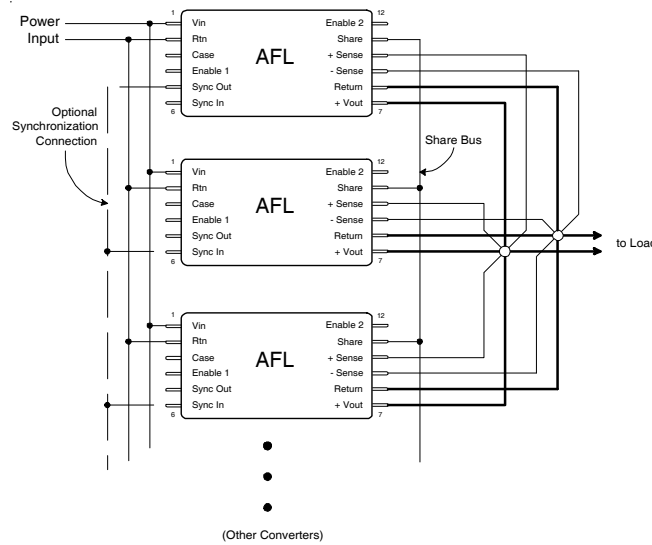
Figure 3. Preferred Connection for Parallel Operation
