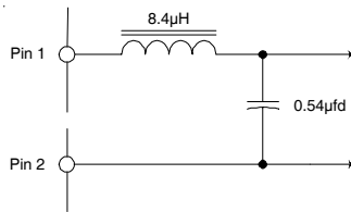
Figure 4. Input Filter Circuit
