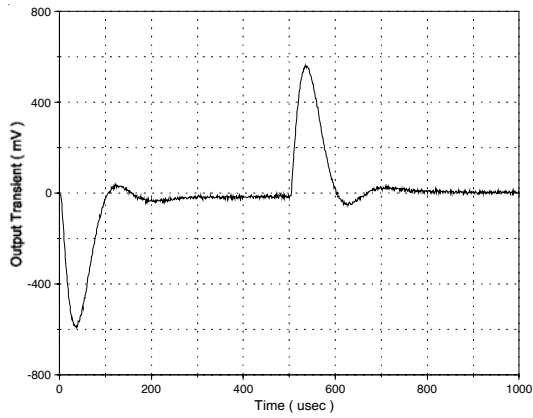
Fig.28 Output Load Transient Response 50% Load to/from 100% Load
