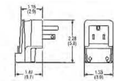
Right Angle Plug
