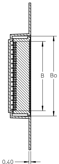
SECTION Y-Y
