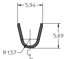
SECTION A-A INSULATION CRIMP
