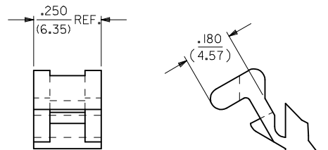
DETAIL 4 .093/(2.36) PREBENT MOUNTING EAR
