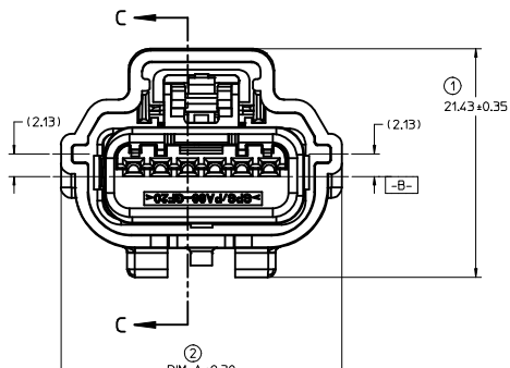
POLARIZATION A FRONT VIEW
