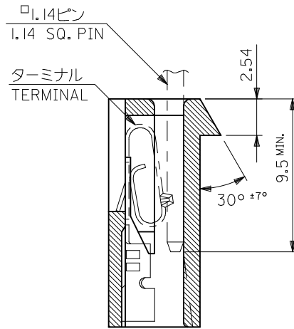
SECT. C-C
