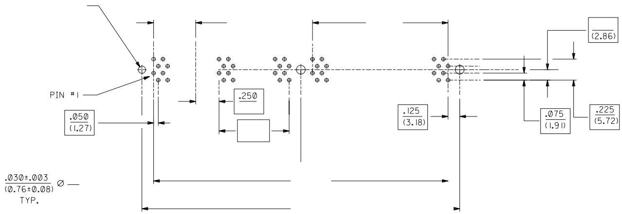
P.C. BOARD HOLE PATTERN (CONNECTOR SIDE)
