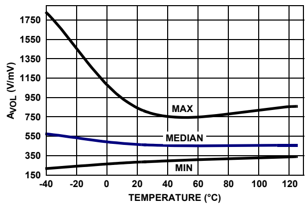
FIGURE 29. A_{VOL} vs TEMPERATURE R_L = 100k, V_+, V_- = \pm 2.5V, V_0 = -2V \text{ TO } +2V
