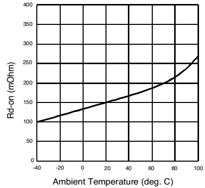
Figure 4. Typical On-Resistance
