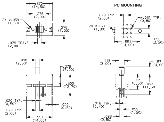
OS202011MV4QN1 DPDT
