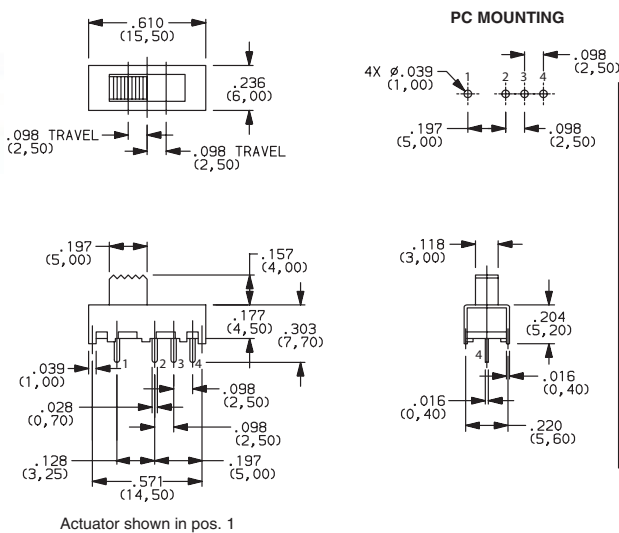
OS103012MU2QP1 SP3T
