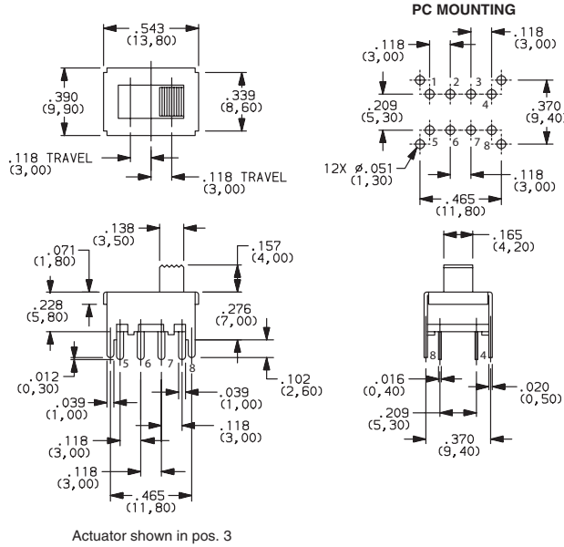
OS203013MT6QN1 DP3T
