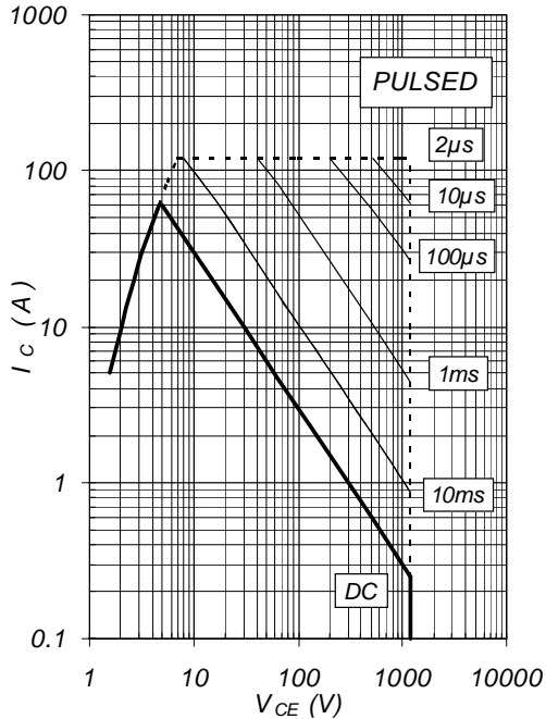
Fig.3 - Forward SOA T_C=25^\circ\text{C}; T_J < 150^\circ\text{C}
