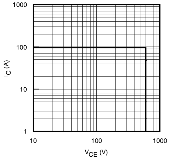
Fig. 4 - Reverse Bias SOA T_J = 175^{\circ} C; V_{GE} = 20V
