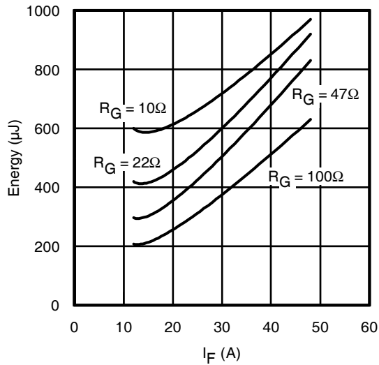
Fig. 21 - Typ. Diode E_{RR} vs. I_F T_J = 175^{\circ}C
