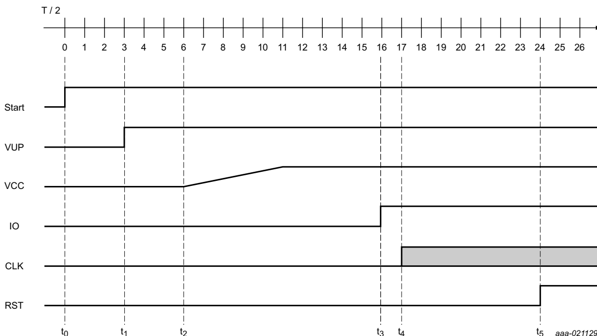
Fig 9. Contact interface - activation sequence
