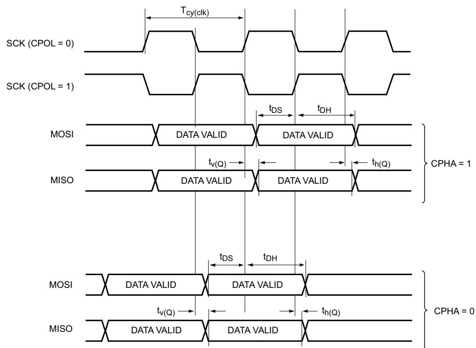
Fig 39. SPI slave timings
