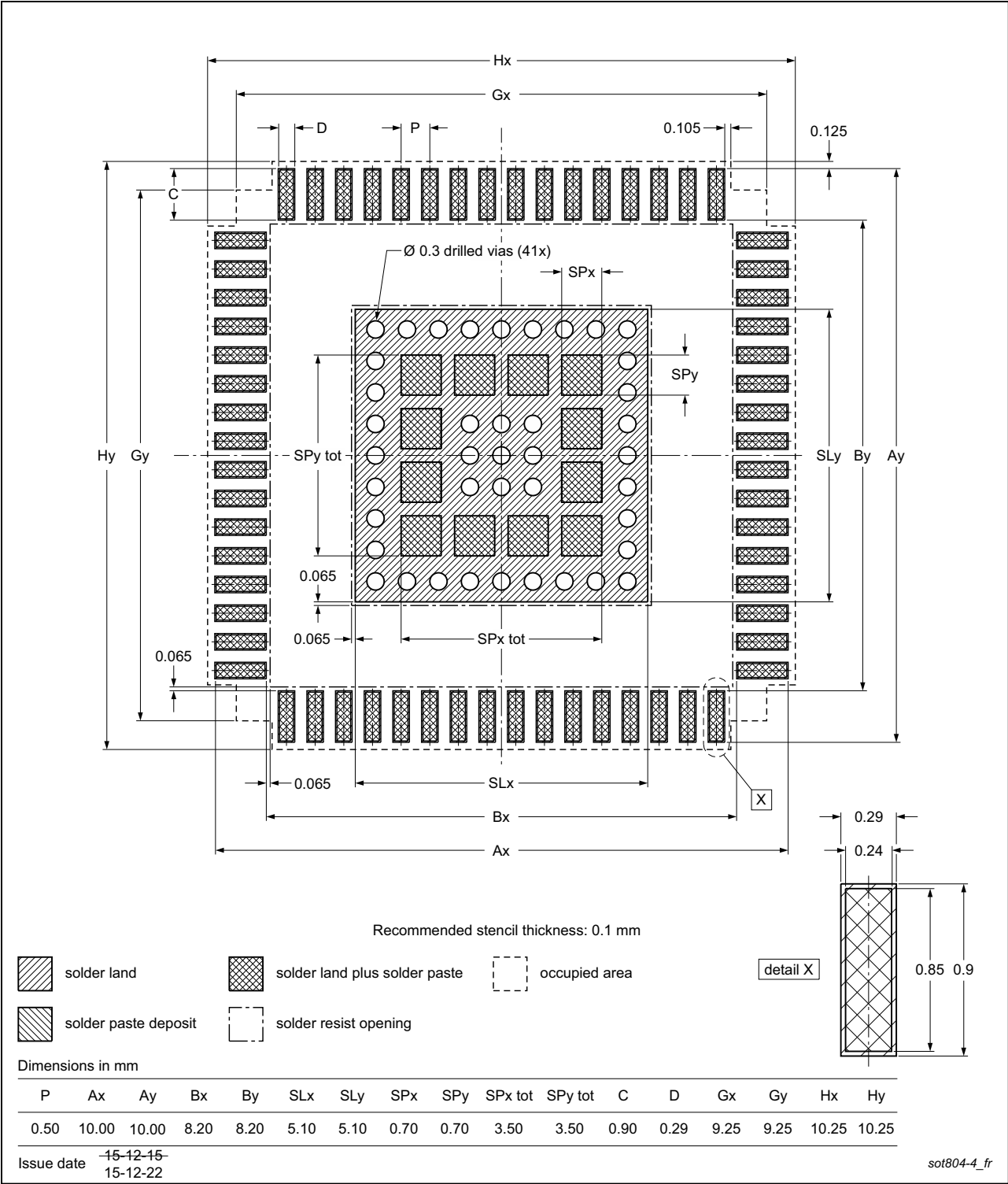
Fig 44. Footprint information for reflow soldering of HVQFN64
