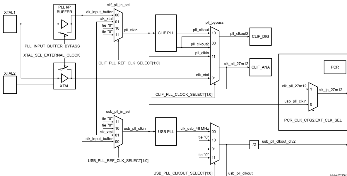
Fig 23. Clocks and IP overview
