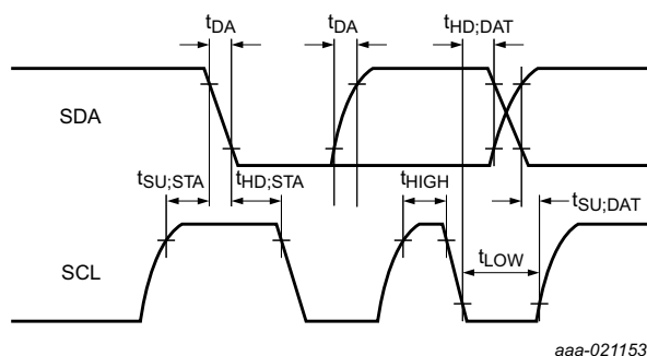
Fig 38. I 2 C-bus pins clock timing
