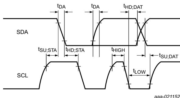
Fig 36. I 2 C-bus pins clock timing
