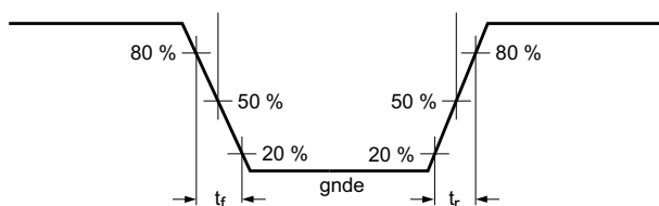
Fig 35. Output timing measurement condition for GPIO
