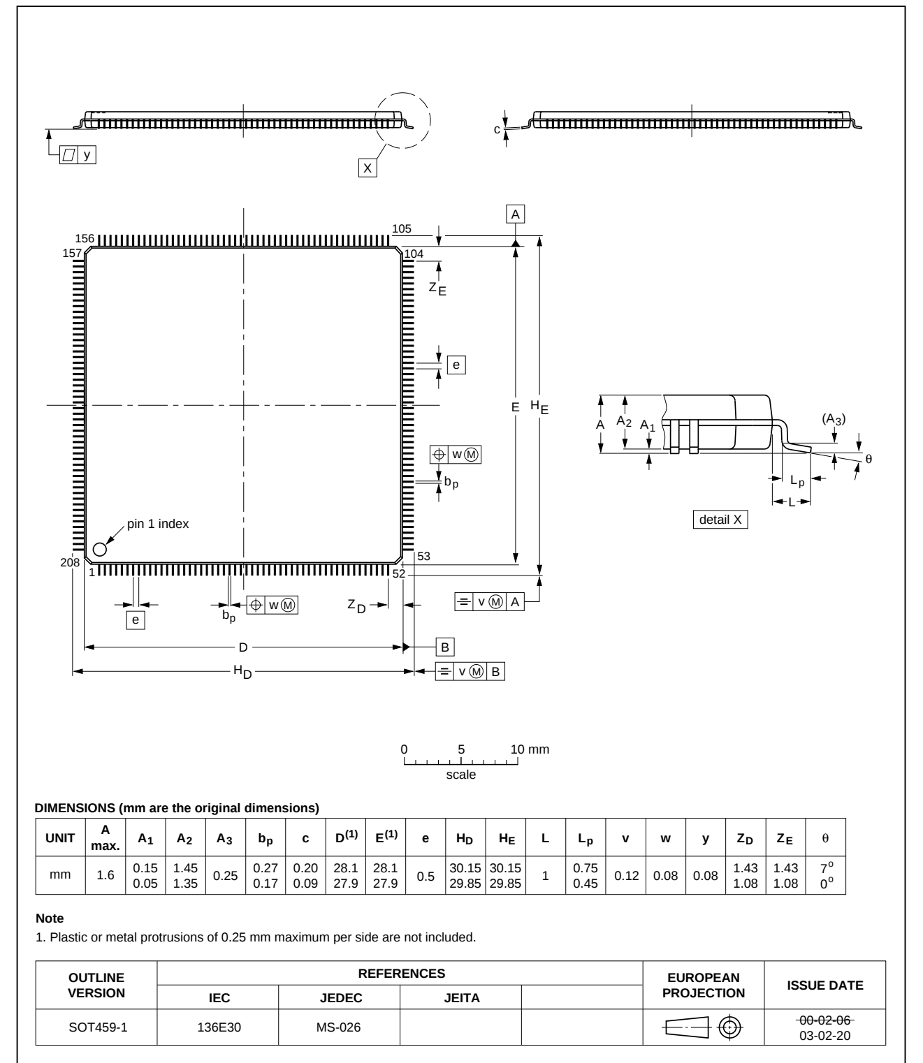
Fig 51. Package outline of the LQFP208 package
