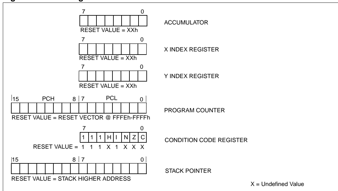
Figure 7. CPU registers
