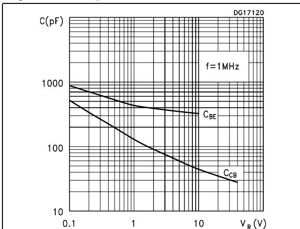
Figure 8. Capacitances
