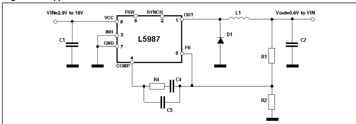
Figure 1. Application circuit
