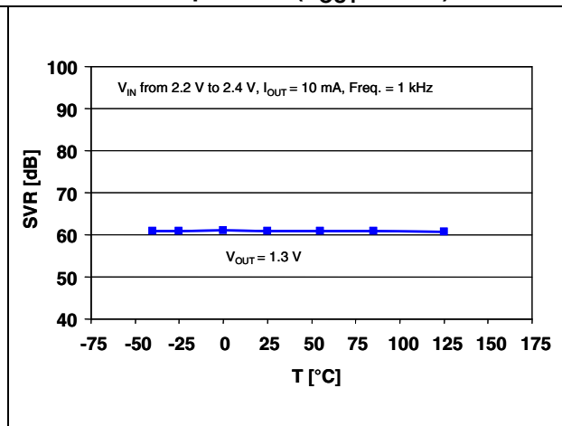
Figure 21. Supply voltage rejection vs. temperature ( V_{OUT} = 1.3\text{ V} )
