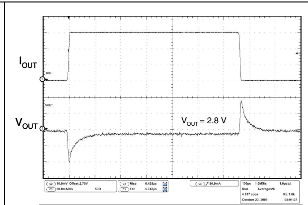
Figure 35. Load transient ( V_{OUT} = 2.8\text{ V} )
