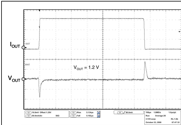
Figure 34. Load transient ( V_{OUT} = 1.2\text{ V} )
