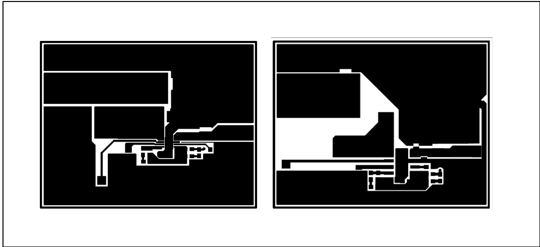
Figure 19. PCB layout: L7985 and L7985A (component side)
