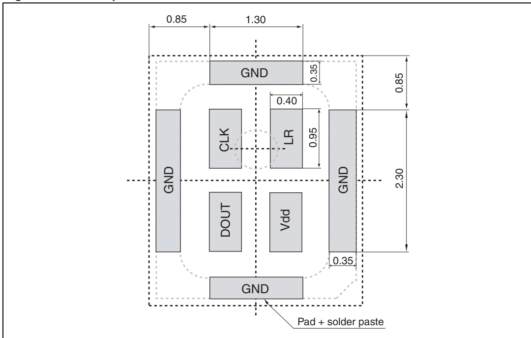
Figure 6. Land pattern
