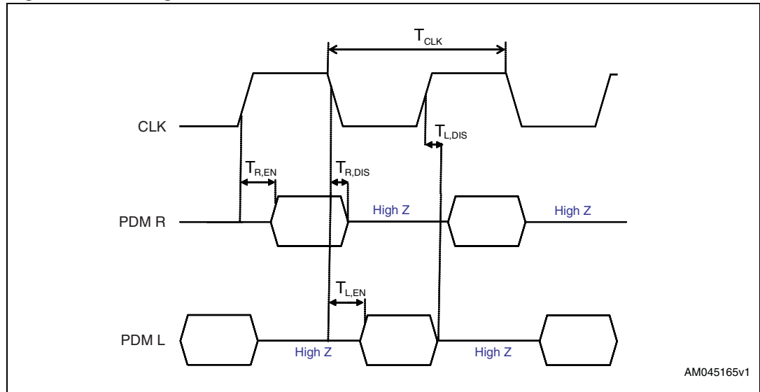
Figure 2. Timing waveforms
