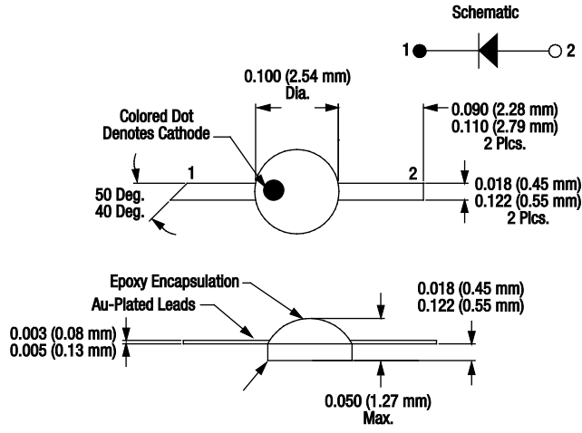
Figure 13. -250 Package Dimensions
