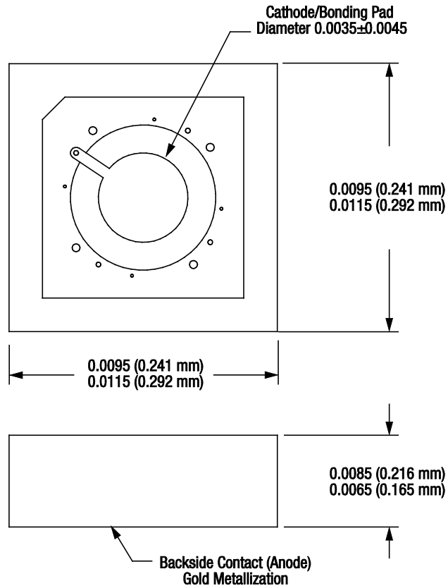
Figure 15. 571-006 Package Dimensions
