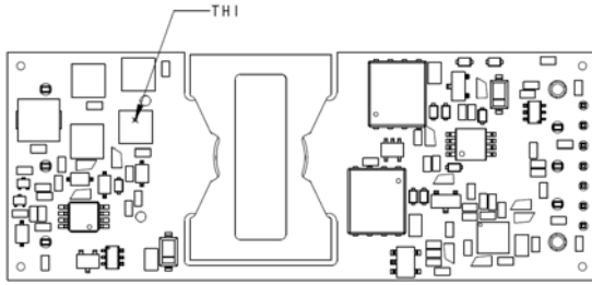
Figure 18. Location of the thermal reference temperature TH1.
