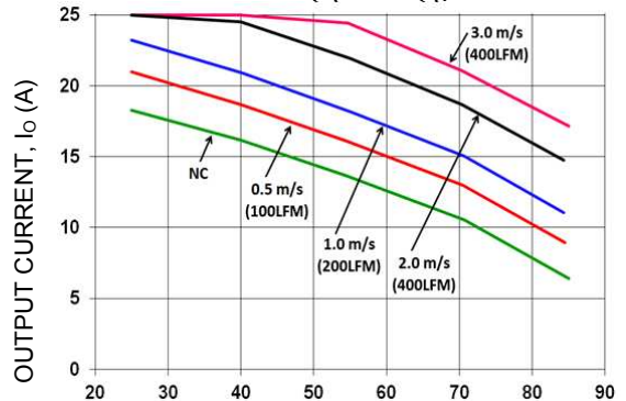
Figure 21. Output Current Derating for the Base plate EBDW025A0B-H in the Transverse Orientation; Airflow Direction from Vin(+) to Vin(-); Vin = 48V.
