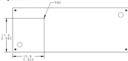
Figure 19. Location of the thermal reference temperature TH2 for Baseplate module.
