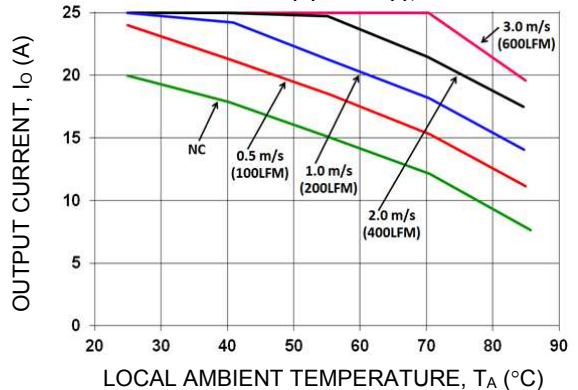
Figure 22. Output Current Derating for the Base Plate EBW025A0Bxx-H and 0.25” heat sink in the Transverse Orientation; Airflow Airflow Direction from Vin(-) to Vin(+); Vin = 48V.
