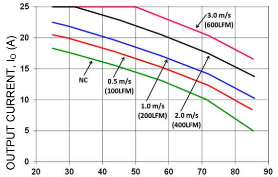
Figure 20. Output Current Derating for the Open Frame EBDW025A0B in the Transverse Orientation; Airflow Direction from Vin(+) to Vin(-); Vin = 48V.
