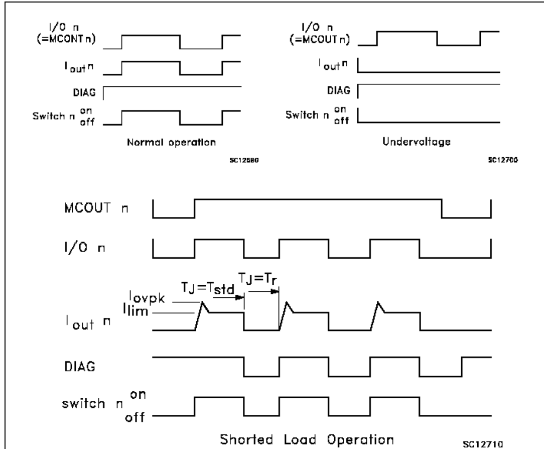
Figure 7. Switching waveforms
