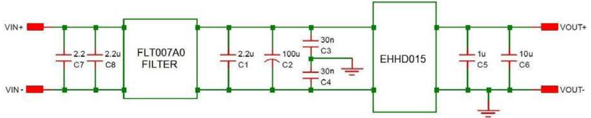
Figure 27. EMC Considerations
