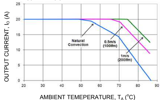
Figure 17. Output Current Derating for the Module with Heatplate; Airflow in the Transverse Direction from V_{out(-)} to V_{out(+)} ; V_{IN} = 48V .
