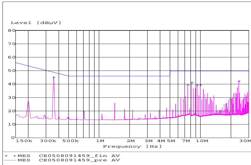
Figure 21. EMC Considerations
