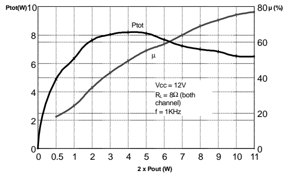
Figure 8. Ptot & Efficiency vs Ouput Power
