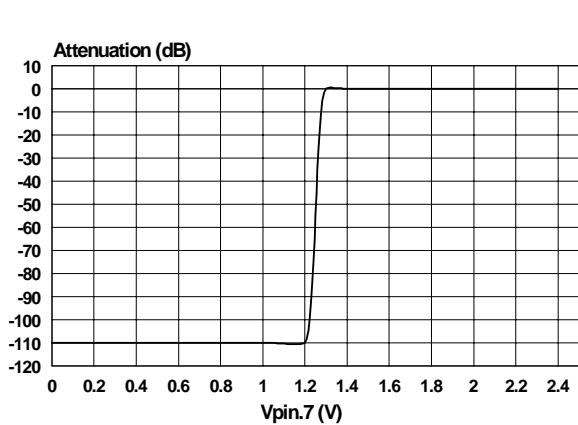
Figure 10. Stand-By attenuation vs Vpin 7
