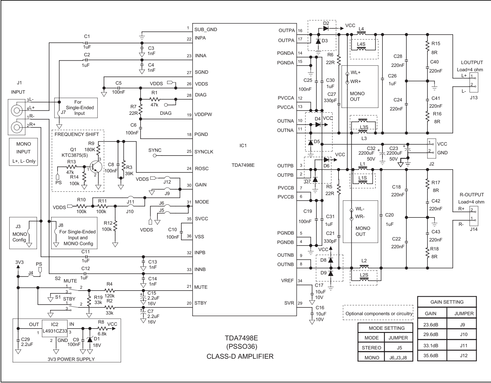
Figure 3. Test circuit stereo application and mono BTL mode
