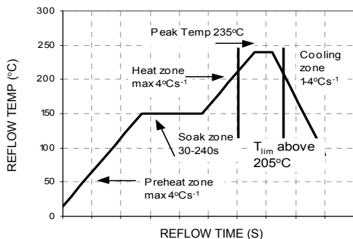
Figure 23. Reflow Profile for Tin/Lead (Sn/Pb) process
