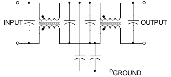
Figure 4. Internal Schematic
