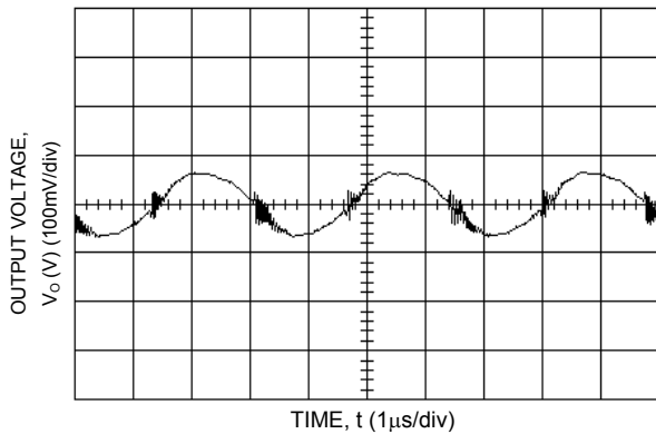
Figure 2. Typical Output Ripple and Noise at Room Temperature and 48Vin; I o = I o,max ; C o,ext = 470μF.
