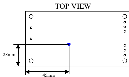
Figure 14. Case ( T_c ) Temperature Measurement Location (top view).
