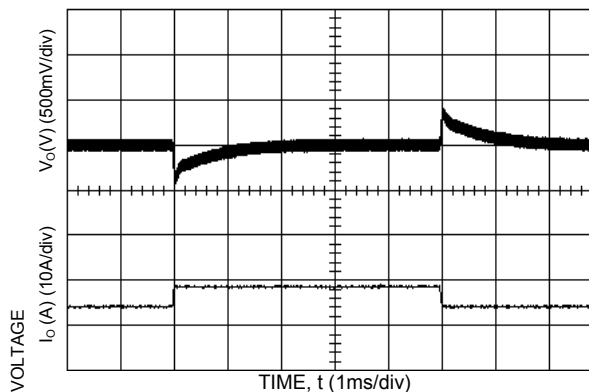
Figure 3. Transient Response to Dynamic Load Change from 25% to 50% to 25% of Full Load at Room Temperature and 48 Vdc Input; 0.1A/μS
