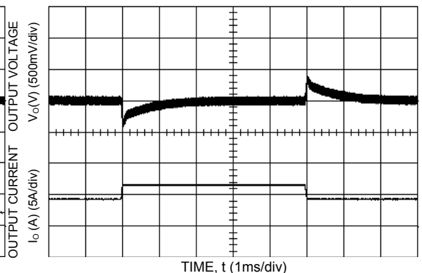
Figure 6. Transient Response to Dynamic Load Change from 50% to 75% to 50% of Full Load at Room Temperature and 48 Vdc Input; 0.1A/μS
