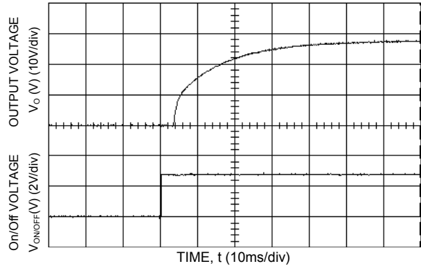
Figure 4. Typical Start-Up Using Remote On/Off, R1=30Kohm; C o,ext = 470μF.
