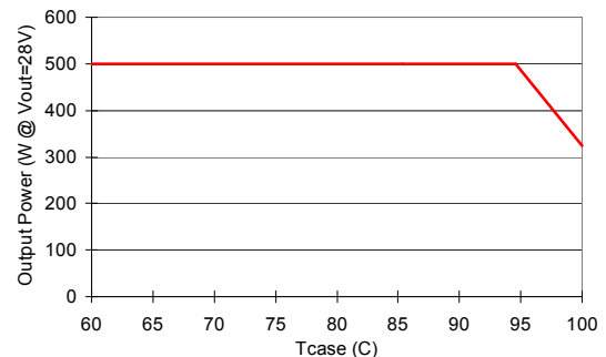
Figure 15. Output Power Derating for FNW500R in Conduction cooling (cold plate) applications; T_a < 72^\circ\text{C} in vicinity of module interior; V_{IN} = V_{IN, NOM}
