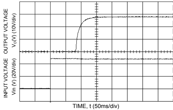
Figure 5. Typical Start-Up Using from V IN , positive logic version shown; C o,ext = 470μF.
