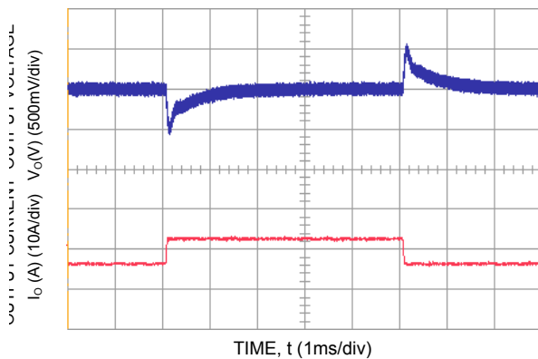
Figure 3. Transient Response to Dynamic Load Change from 25% to 50% to 25% of Full Load at Room Temperature and 48 Vdc Input; 0.1A/uS ; C o,ext = 470μF.
