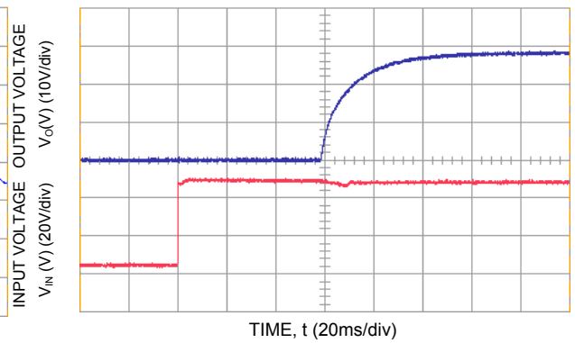
Figure 5. Typical Start-Up Using from V IN , positive logic version shown; C o,ext = 470μF.
