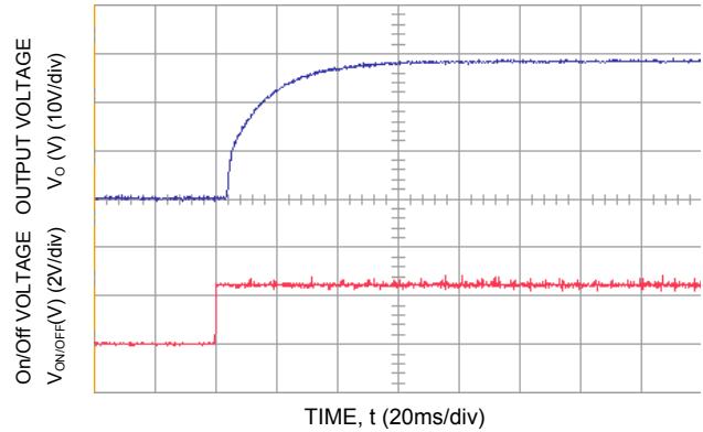
Figure 4. Typical Start-Up Using Remote On/Off, R1=30Kohm; C o,ext = 470μF.
