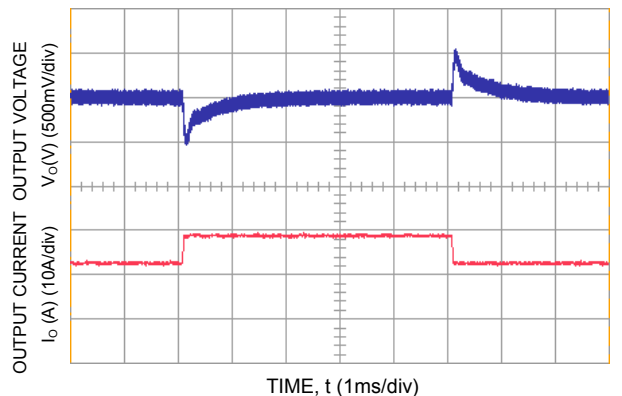
Figure 6. Transient Response to Dynamic Load Change from 50% to 75% to 50% of Full Load at Room Temperature and 48 Vdc Input; 0.1A/uS ; C o,ext = 470μF.
