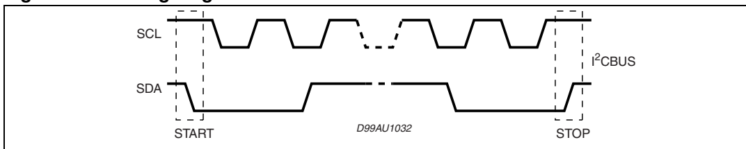
Figure 26. Timing diagram on the I 2 C bus
