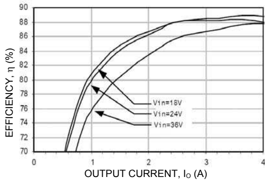
Figure 49. Converter Efficiency versus Output Current.
