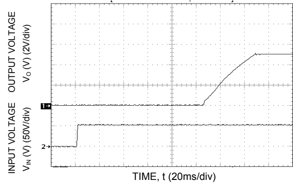
Figure 5. Typical Start-Up with application of Vin.
