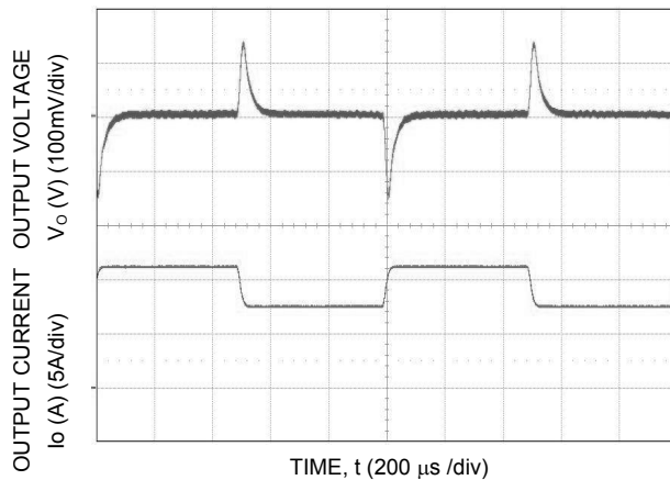
Figure 3. Transient Response to Dynamic Load Change, 1.0A/μS, from 75% to 50% to 75% of full load.
