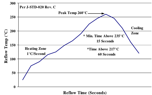
Figure 19. Recommended linear reflow profile using Sn/Ag/Cu solder.
