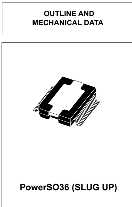
Figure 34. PowerSO36 (slug up) mechanical data and package dimensions
