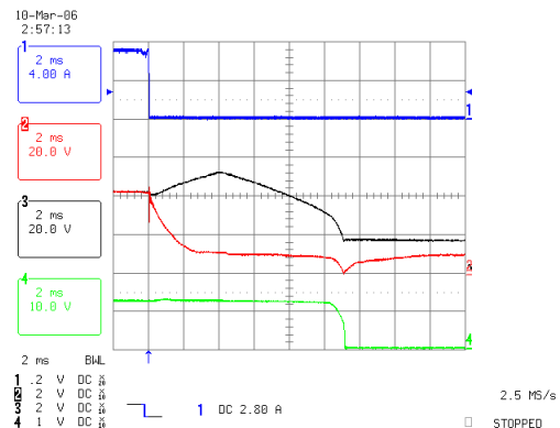
Figure 8. Holdup Performance; Loss of Feed A (with Feed B=0Vdc); Load=QBW CH1: lin(-48V_AF), CH2: 48V_AF, CH3: 48V_OUT, CH4: 12Vout
