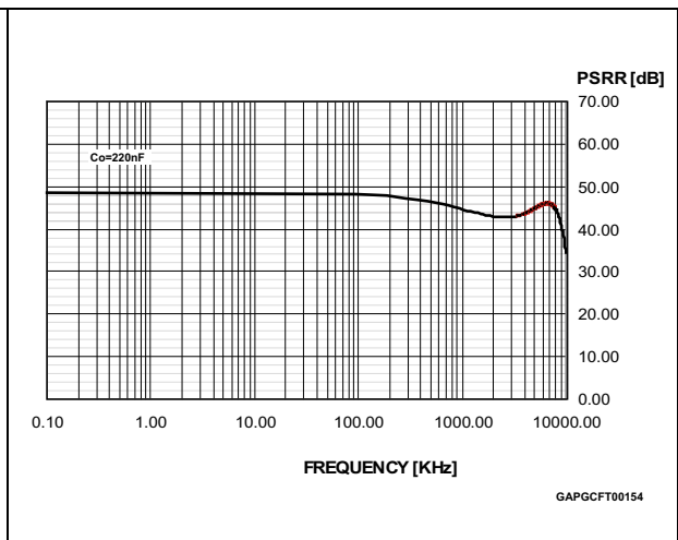
Figure 20. PSRR
