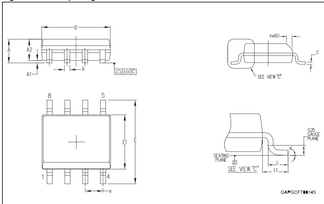
Figure 35. SO-8 package dimensions
