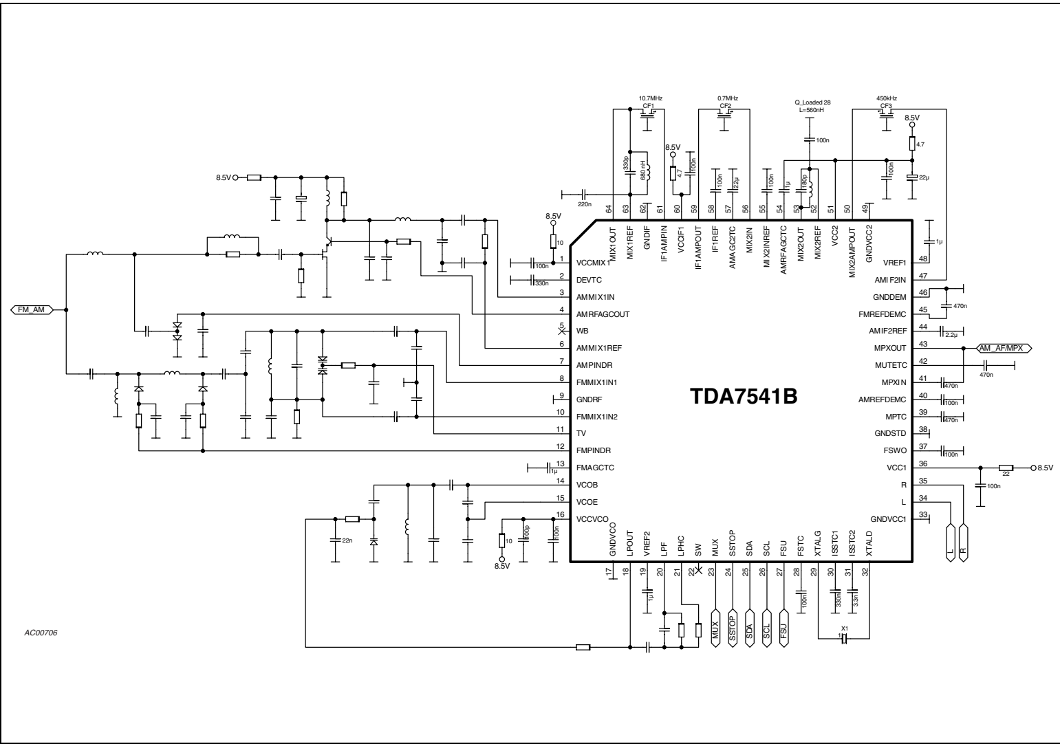
Figure 15. Application circuit
