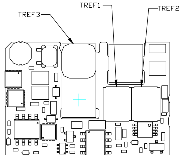
Figure 43. T_{ref} Temperature Measurement Locations.
