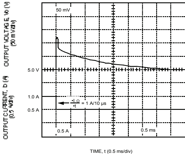
Figure 4. CC025 Dual-Output-Series Typical 5 V Output Voltage Response to a Step Load Change from 50% to 25% of I_{o, \text{max}} at V_i = V_{i, \text{nom}} and T_c = 25\text{ }^\circ\text{C}
