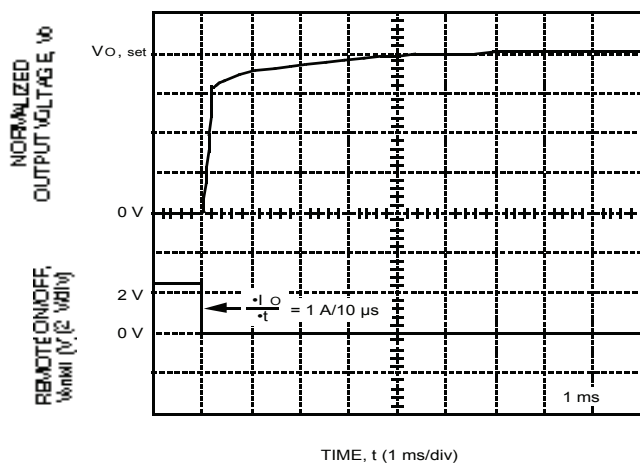
Figure 10. CC025 Dual-Output-Series Typical Output Voltage Rise Time with Remote On/Off at V_i = V_{i, nom} , I_o = 0.8 (I_{o, max}) , and T_c = 25\text{ }^\circ\text{C}
