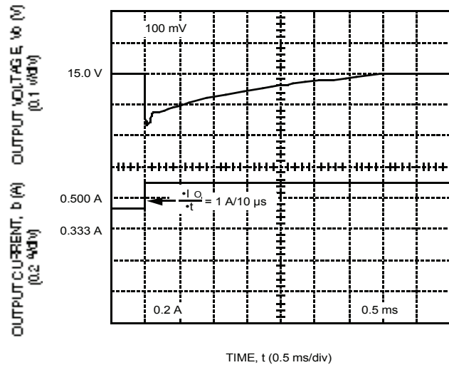
Figure 9. CC025 Dual-Output-Series Typical 15 V Output Voltage Response to a Step Load Change from 50% to 75% of I_{O, max} at V_i = V_{i, nom} and T_c = 25\text{ }^\circ\text{C}
