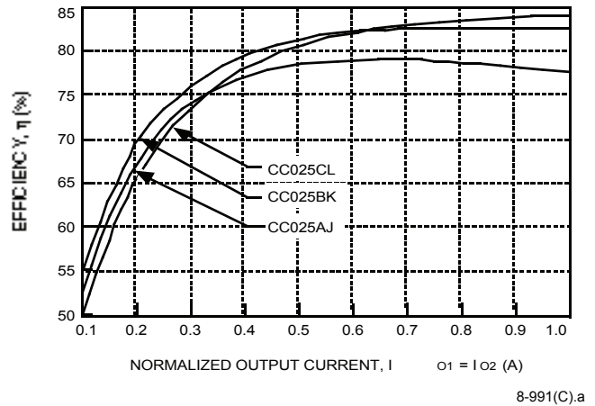
Figure 3. CC025 Dual-Output-Series Efficiency vs. Normalized Output Currents at V_i = 28\text{ V} and T_c = 25\text{ }^\circ\text{C}
