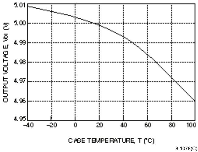
Figure 2. CC025 Triple-Output-Series Typical Output Voltage Variation of 5 V Output Over Ambient Temperature Range
